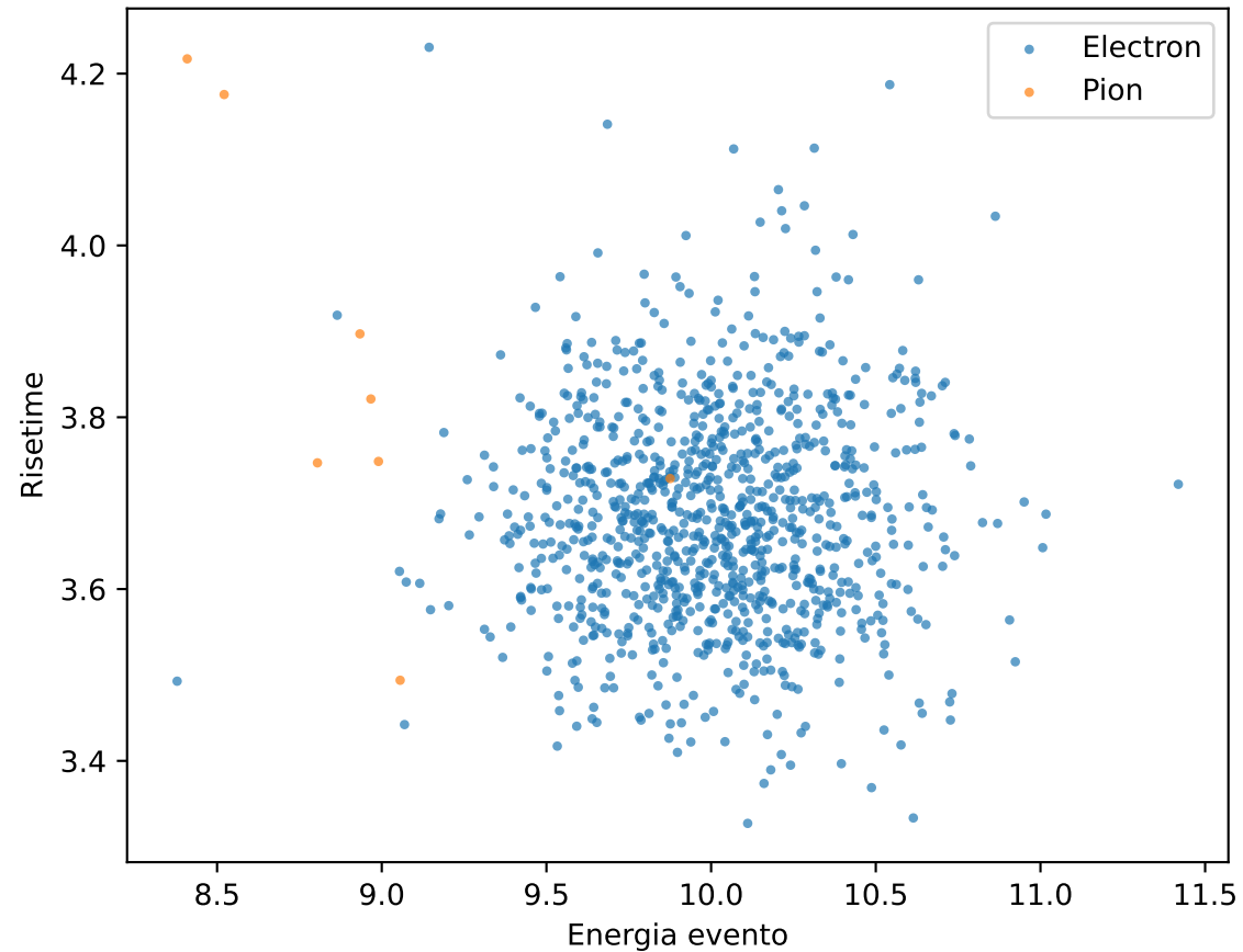
Scatter plot e/pi (cutted) 10.0GeV
