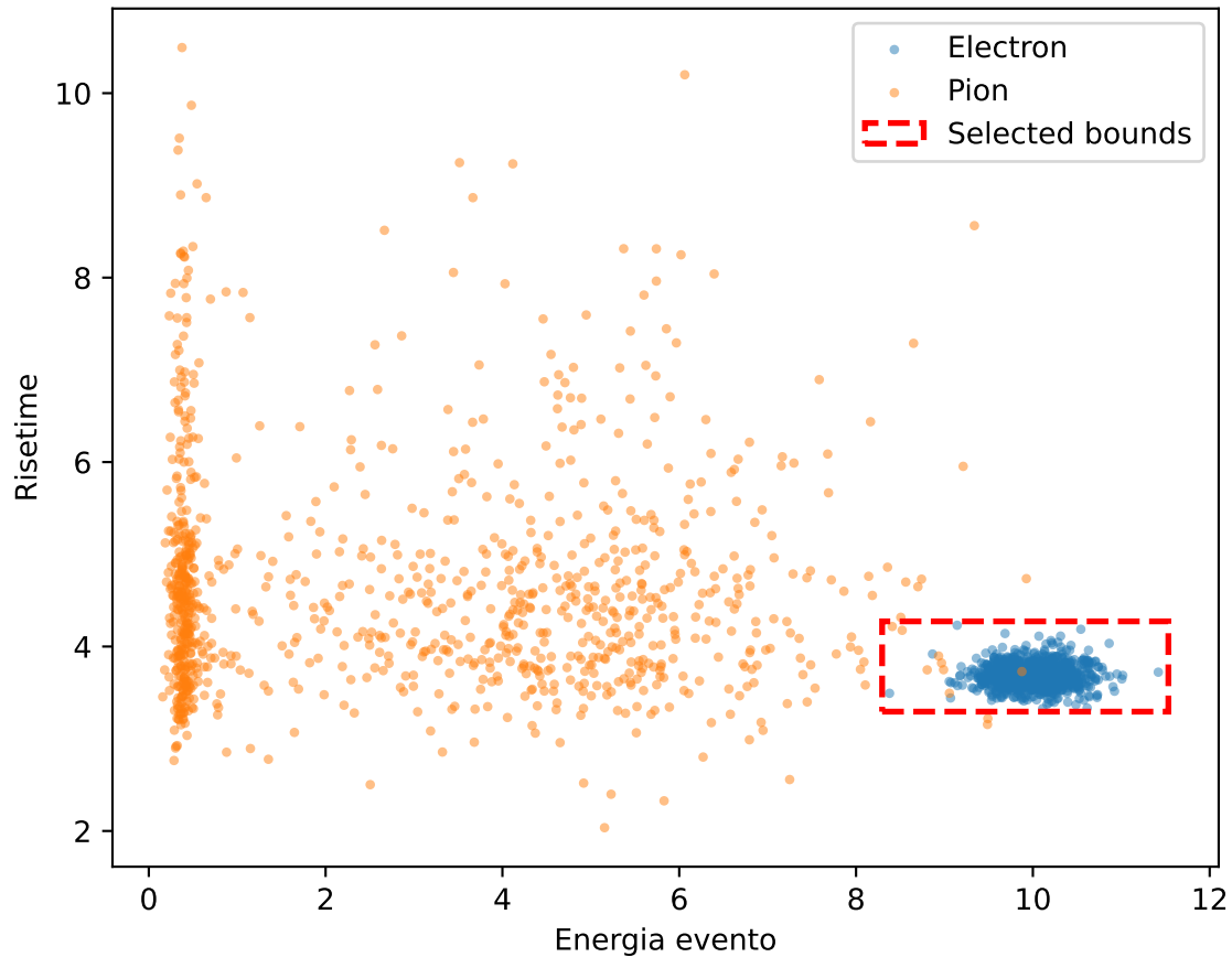
Scatter plot e/pi (all) 10.0GeV
